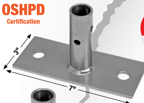
WR-SFP Single Foot Plate
