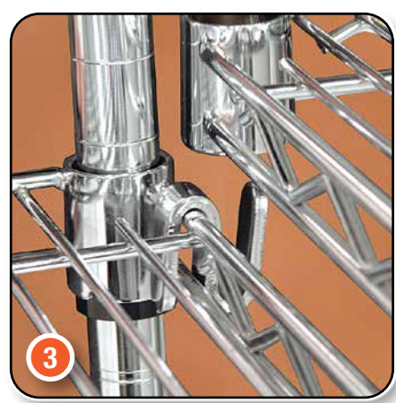
3 Two "S-Hooks" are used to connect add-on wire shelf to starter units.
