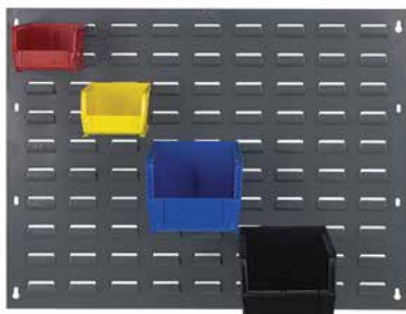
QLP-2721 27-3/4"L x 21"H Accepts all sizes of Ultra and Mesh Bins. Up to 175 lb. load capacity. (Bins sold separately)
