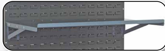
SLP-1236 (12"D x 36"W) and SLP-1836 (18"D x 36"W) Flat Shelf with 2 Brackets. Available in 12" or 18" Depth. Up to 75 lb. load capacity
